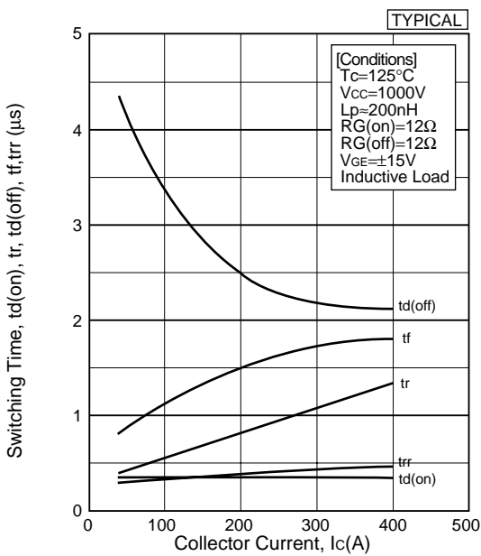
Switching time vs. Collector current
