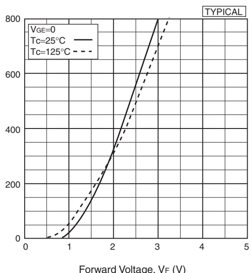
Forward voltage of free-wheeling diode
