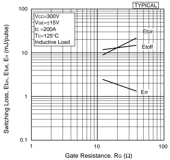
Switching loss vs. Gate resistance
