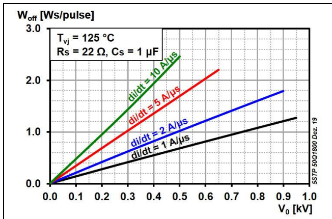
Fig. 13 Typical turn-off energy, rectangular waves
